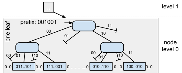
Figure 4. Internal structure of a leaf node of a briere.
