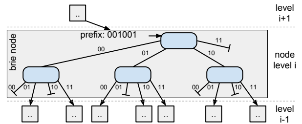
Figure 3. Internal structure of an inner node of a briere.
